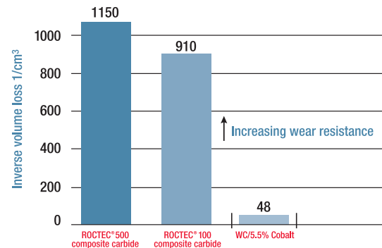
ASTM B-611 Abrasion Slurry
